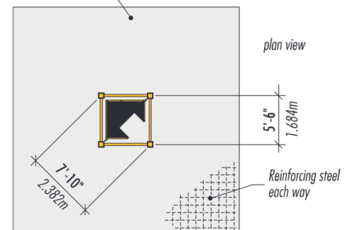
FOUNDATION DETAILS with 100 LC tower anchored in reinforced concrete slab
